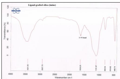
Fig. 2. FTIR of ligand-grafted silica (imine)
