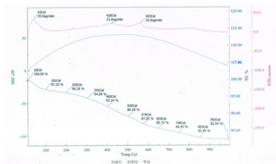
Fig. 4. TGA of SiO 2 -Co(OAc) 2
