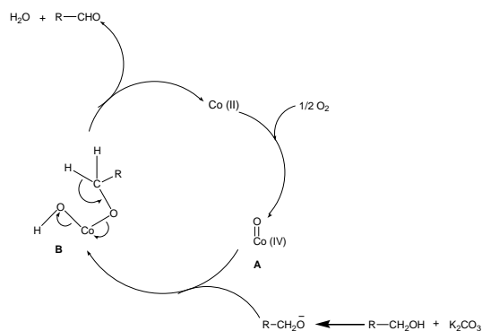
Fig. 8. Proposed mechanism for the oxidation of alcohols to corresponding aldehydes using SiO_2-Co(OAc)_2 in the presence of oxygen
