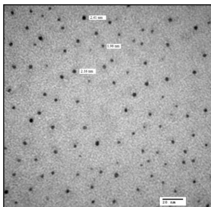
Fig. 6. TEM Micrograph of \text{SiO}_2\text{-Co(OAc)}_2
