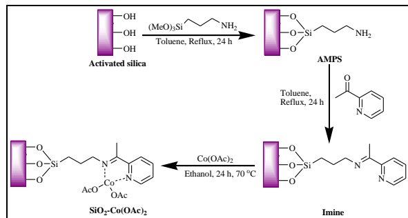
Fig. 1. Preparation of silica-functionalized cobalt(II) acetate [SiO 2 -Co(OAc) 2 ]
