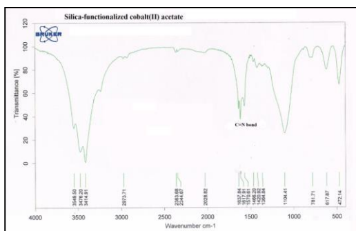
Fig. 3. FTIR of SiO 2 -Co(OAc) 2
