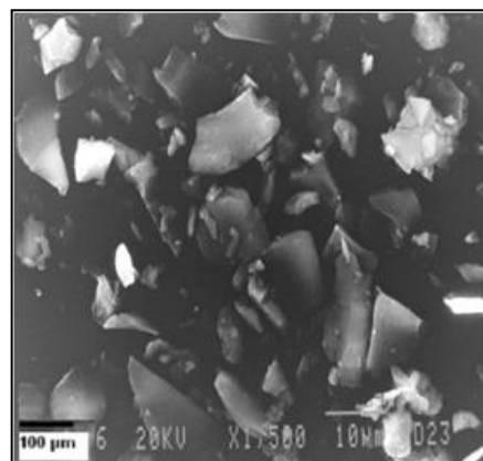
Fig. 5. SEM image of SiO 2 -Co(OAc) 2
