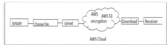
Fig. 3. Flow diagram
