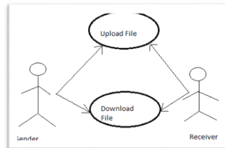
Fig. 2. Use-case diagram
