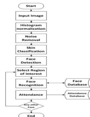
Fig8: Algorithm of automatic attendance using face recognition
